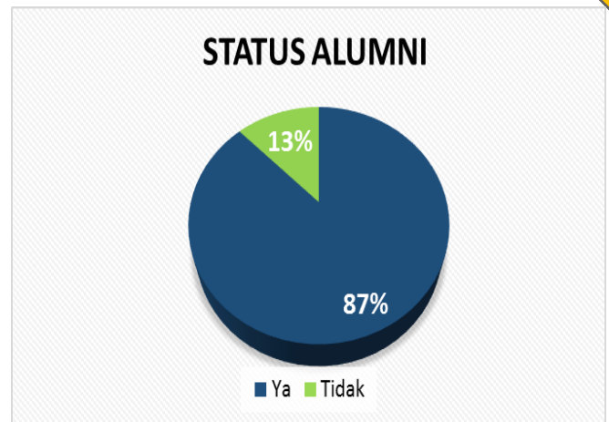
Gambar 8. Status Alumni
